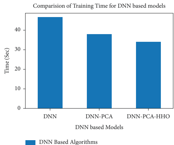
FIGURE 15: Training time analysis for DNN-based models.
